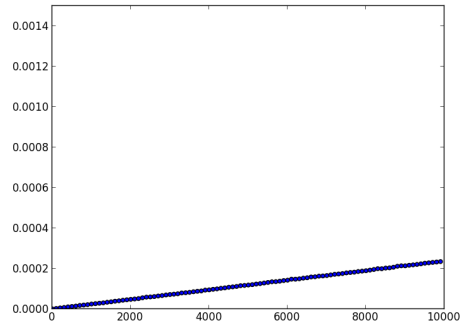
FIGURE 1: n = 10\,000 , \text{range}(n, 0, -1)
