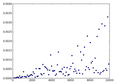
FIGURE 3: n = 10\,000 , \text{randlist}
