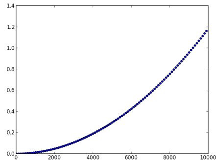
FIGURE 2: n = 10\,000 , \text{range}(n)
