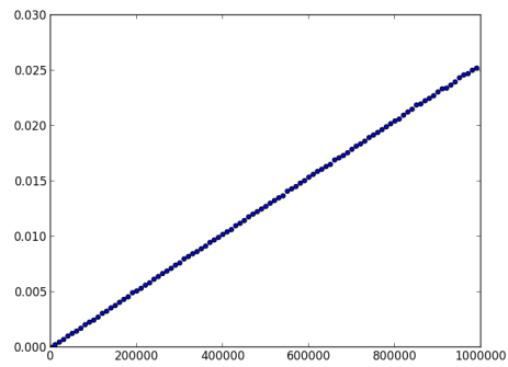
FIGURE 4: n = 1\,000\,000 , \text{range}(n, 0, -1)
