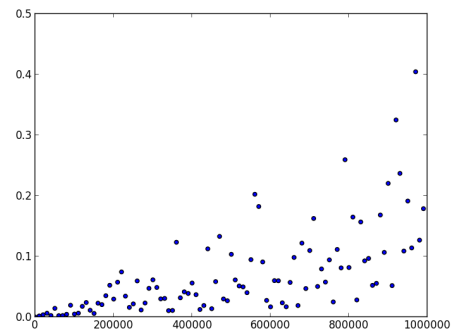
FIGURE 5: n = 1\,000\,000 , \text{randlist}
